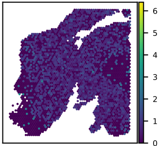
SNU24A SLC35B4 expression Moran's I = 0.06
