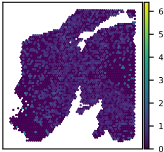
SNU24A METTL8 expression Moran's I = 0.05
