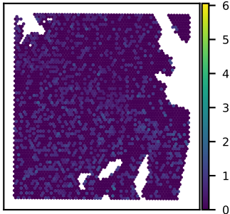
SNU51A GAS2L3 expression Moran's I = 0.04
