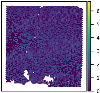
SNU43A CTNNBIP1 expression Moran's I = 0.03
