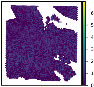
SNU24B POMT2 expression Moran's I = 0.03
