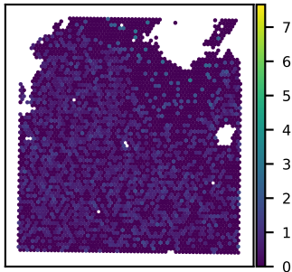
SNU21B C6orf226 expression Moran's I = 0.02
