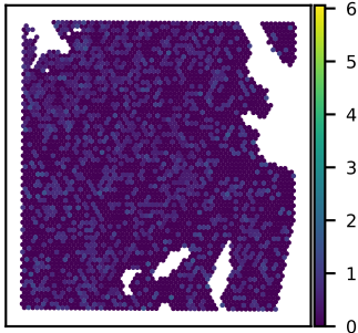
SNU51A DDX52 expression Moran's I = 0.02
