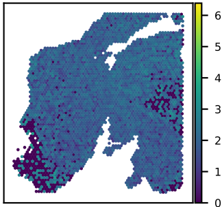
SNU24A PTTG1IP expression Moran's I = 0.19
