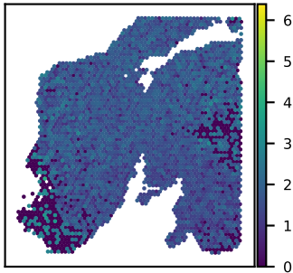
SNU24A RNF13 expression Moran's I = 0.13
