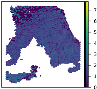
SNU18A ATXN10 expression Moran's I = 0.19
