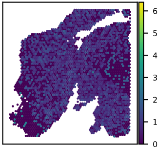
SNU24A FUNDCl expression Moran's I = 0.08
