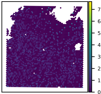
SNU21B C6orf136 expression Moran's I = 0.01
