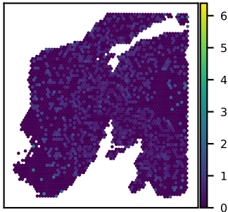
SNU24A PCDHGA11 expression Moran's I = 0.02
