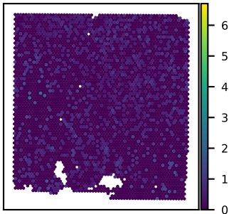
SNU43A HDHD3 expression Moran's I = 0.01
