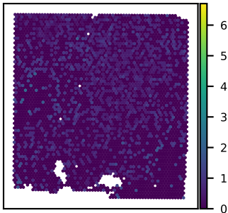
SNU43A REEP4 expression Moran's I = 0.02
