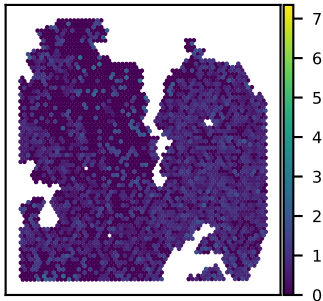
SNU27B SLC12A9 expression Moran's I = 0.07
