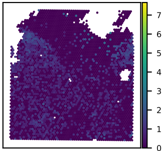
SNU21B C21orf62 expression Moran's I = 0.22
