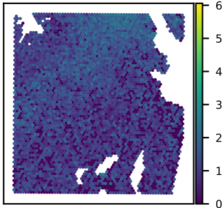
SNU51A CLDND1 expression Moran's I = 0.23
