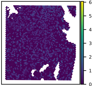
SNU51A FGFR2 expression Moran's I = 0.03
