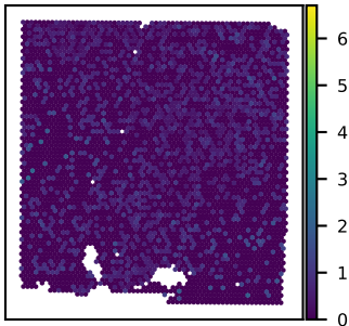
SNU43A SLC35G2 expression Moran's I = 0.01
