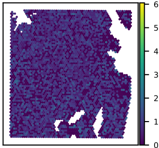
SNU51A HDAC7 expression Moran's I = 0.02
