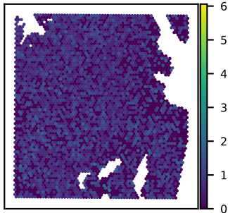
SNU51A GALNT1 expression Moran's I = 0.04
