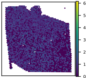
SNU27A ARFGAP3 expression Moran's I = 0.05
