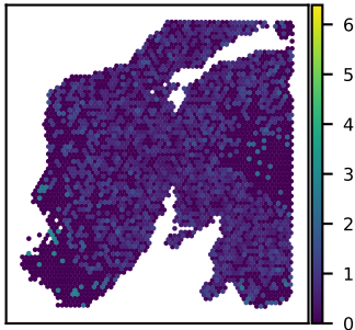
SNU24A SLC41A3 expression Moran's I = 0.05
