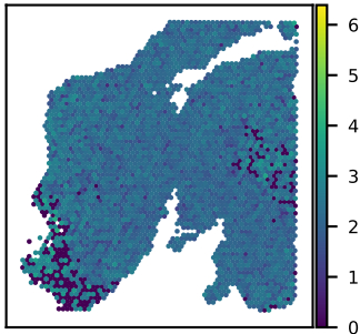
SNU24A GABARAPL2 expression Moran's I = 0.10
