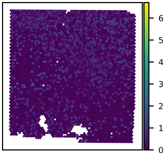
SNU43A PCDHB13 expression Moran's I = 0.06
