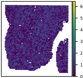
SNU25B TUBG2 expression Moran's I = 0.02
