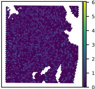
SNU51A SLC10A7 expression Moran's I = 0.02
