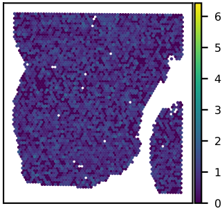
SNU25B PSMA5 expression Moran's I = 0.02
