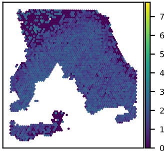
SNU18A SCARB2 expression Moran's I = 0.32
