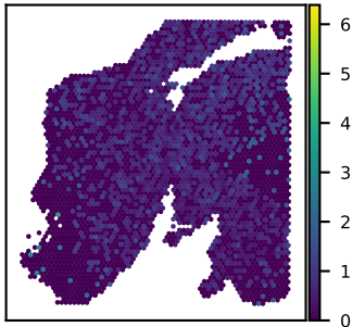
SNU24A GIMAP8 expression Moran's I = 0.07
