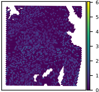
SNU51A KIF11 expression Moran's I = 0.06
