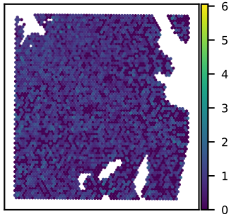
SNU51A ARL4A expression Moran's I = 0.04
