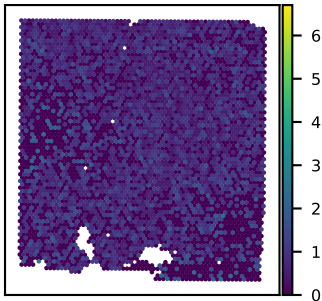
SNU43A KCTD5 expression Moran's I = 0.01
