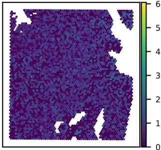
SNU51A SMIM13 expression Moran's I = 0.02
