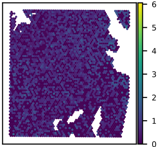
SNU51A ZMYND11 expression Moran's I = 0.04
