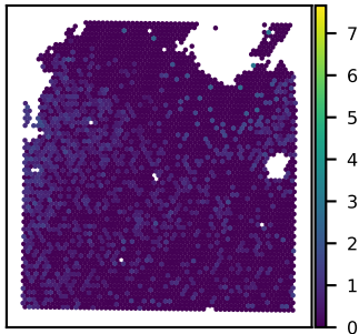
SNU21B SEMA6D expression Moran's I = 0.14
