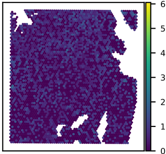
SNU51A HIPK3 expression Moran's I = 0.05
