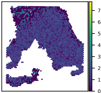
SNU18A WDR26 expression Moran's I = 0.15
