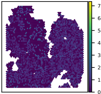
SNU27B ST6GALNAC4 expression Moran's I = 0.06
