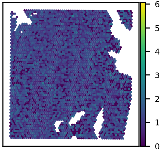
SNU51A SUPT5H expression Moran's I = 0.00
