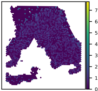
SNU18A VPS37C expression Moran's I = 0.06
