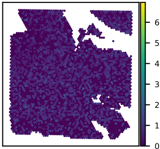
SNU24B TMEM185B expression Moran's I = 0.02
