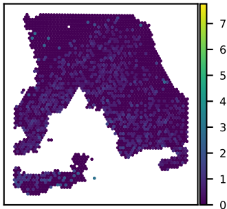
SNU18A ARHGAP33 expression Moran's I = 0.07
