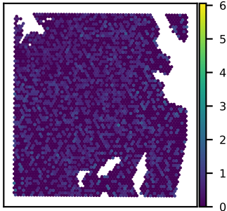
SNU51A SCAF8 expression Moran's I = 0.01
