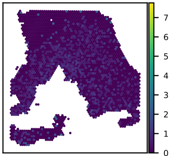
SNU18A KLHL4 expression Moran's I = 0.06
