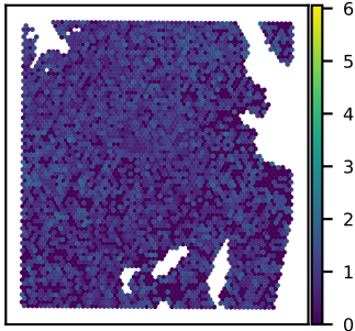
SNU51A PTTG1IP expression Moran's I = 0.06
