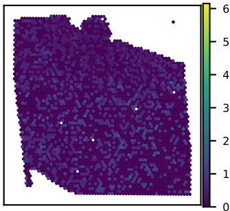
SNU27A FTCDNL1 expression Moran's I = 0.01
