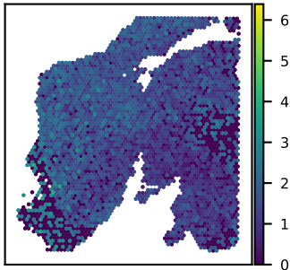
SNU24A CHI3L2 expression Moran's I = 0.16
