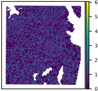
SNU51A MAPKAP1 expression Moran's I = 0.02
